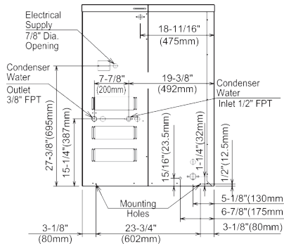
WATER-COOLED UNIT
