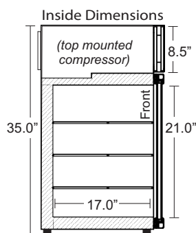
SCTF-4 (side view) 19.8" W x 17.0" D x 21.0" H Door Glass 21.5" W x 22.0" H
