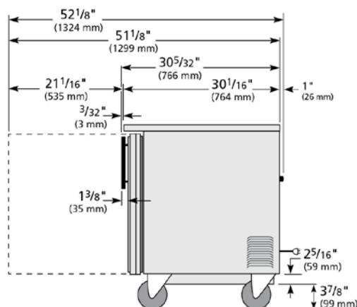
RIGHT VIEW
