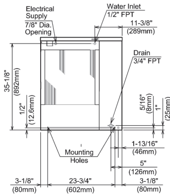
AIR-COOLED UNIT
