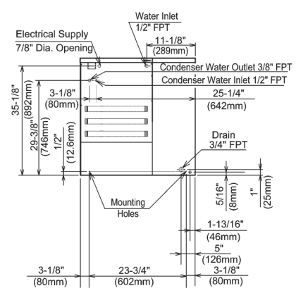
WATER-COOLED UNIT
