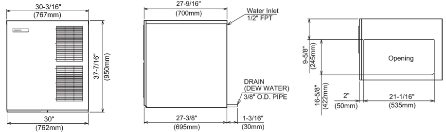
FRONT VIEW
