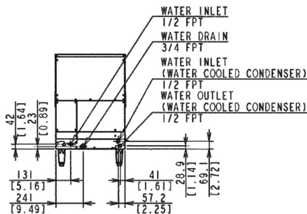
BACK VIEW / AIR-COOLED UNIT
