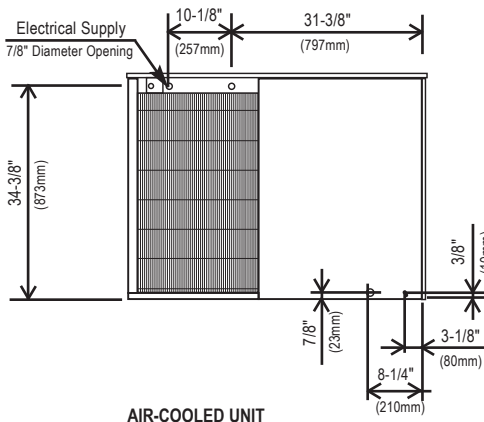
AIR-COOLED UNIT
