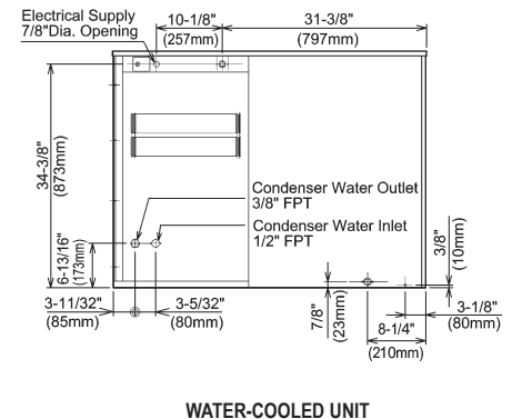
WATER-COOLED UNIT
