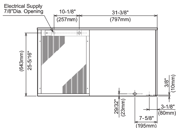
AIR-COOLED UNIT
