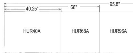
PLAN VIEW
