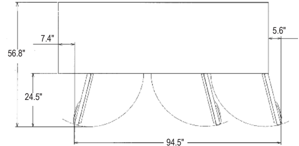
HUR96A (DOOR SWING)
