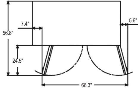
HUR68A (DOOR SWING)
