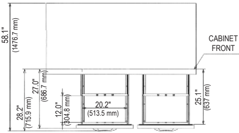
HUR68A-D (TOP VIEW)
