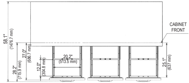
HUR96A-D (TOP VIEW)
