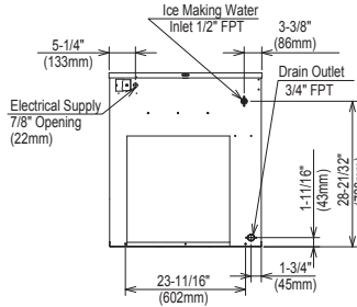
AIR-COOLED UNIT
