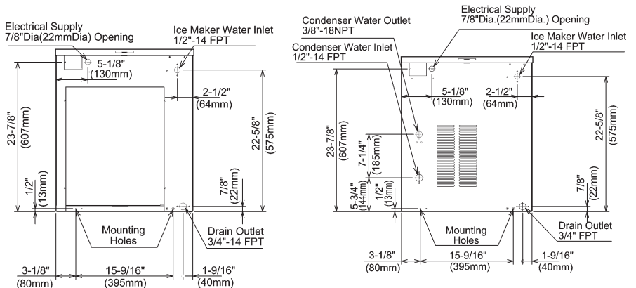
AIR-COOLED UNIT
