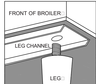
Figure 1 - Leg Placement
