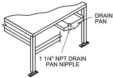
REAR VIEW / DRAIN PAN DETAIL
