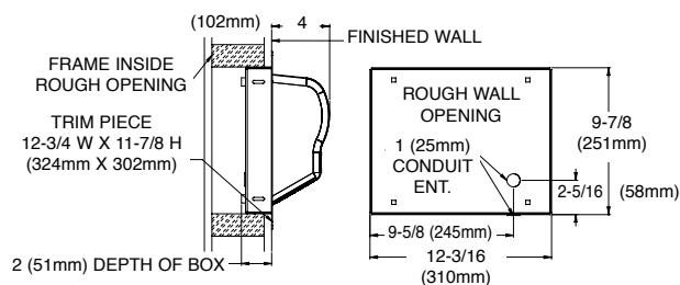
Figure 2 - EXT-MR Series Recessed Mount
